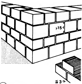
⑦ Ashlar walling
